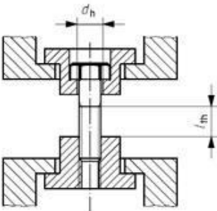
a) Example of testing device for bolts
