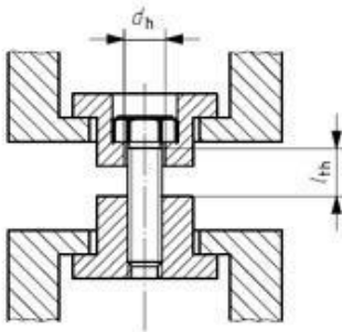
b) Example of testing device for screws
