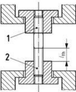
c) Example of testing device for studs
